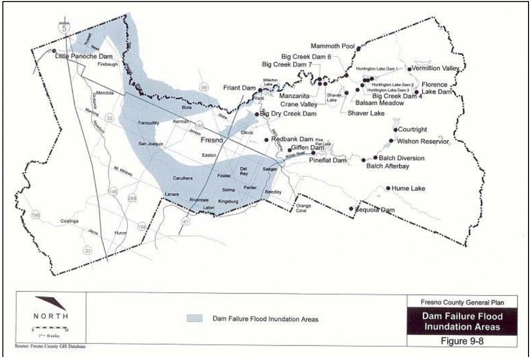
Figure 10: Dam Failure Flood Inundation Area in Fresno County (Source: Fresno County General Plan Background Report 2000)
