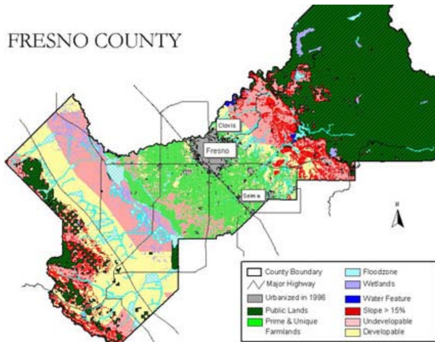
Figure 4: Land use map of Fresno County. While most of the eastern part of the county is public land, central and western portions are developed or farmlands (Source: Desert Research Institute) 18
