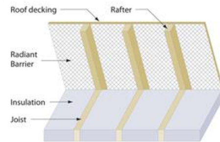
Laminated to underside of roof decking
