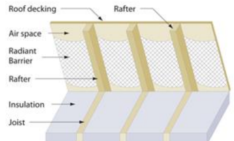
Draped over rafters before decking is installed
