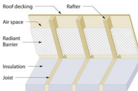
Stapled to sides of rafters or truss top chords
